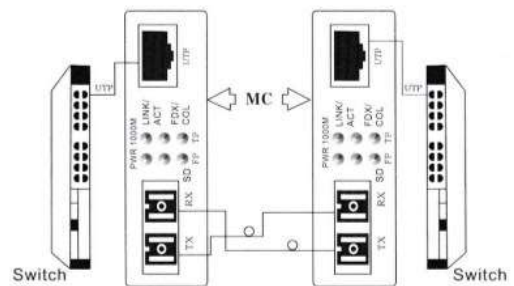
figure: Installation and Connections
